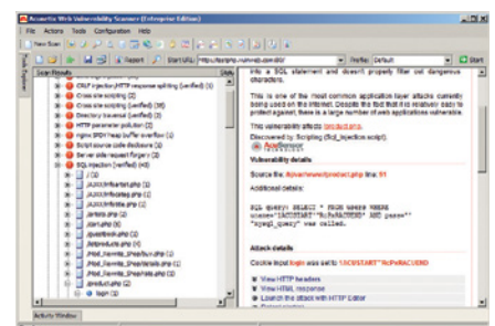
SQLi showing SQL Query (thanks to AcuSensor)
